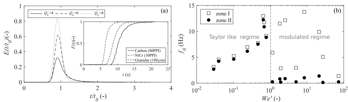
Figure 2: (a) Typical global hydrodynamics results. Modeling of the retention time distribution, E(t/t_0) , and effect of liquid flow rate ( \text{cm}^3/\text{min} ) on curve shape at a constant gas flow rate ( Q_G = 10 \text{ cm}^3/\text{min} ). Inset: Experimental cumulative retention time distribution, F(t) , for different porous medium structures. (b) Local hydrodynamics study, pulsed regime transition at the entrance of the porous medium. The signal main frequency, f_0 , at the entrance of the porous medium, displays a clear regime transition as a function of a modified Weber number.
